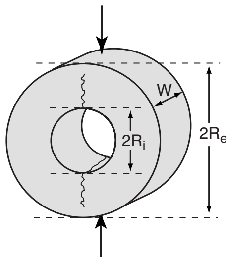
FIG. 1. Schematic view of the toroidal sample (outside radius 60 mm, inside radius 25 mm) and of forces applied during the modified Brazilian test.
