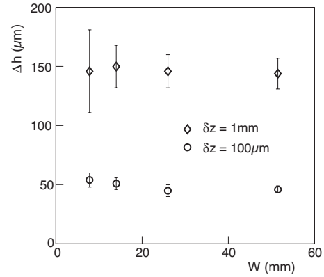
FIG. 8. Height-height correlation function \Delta h(\delta z) for fixed values of \delta z as a function of the specimen width W . ( \diamond ): \delta z=1 mm and ( \circ ): \delta z=100 \mu\text{m} . Error bars: Standard deviation of \Delta h(\delta z) .
